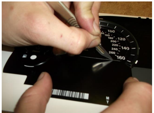
Cut the bottom edge as shown
